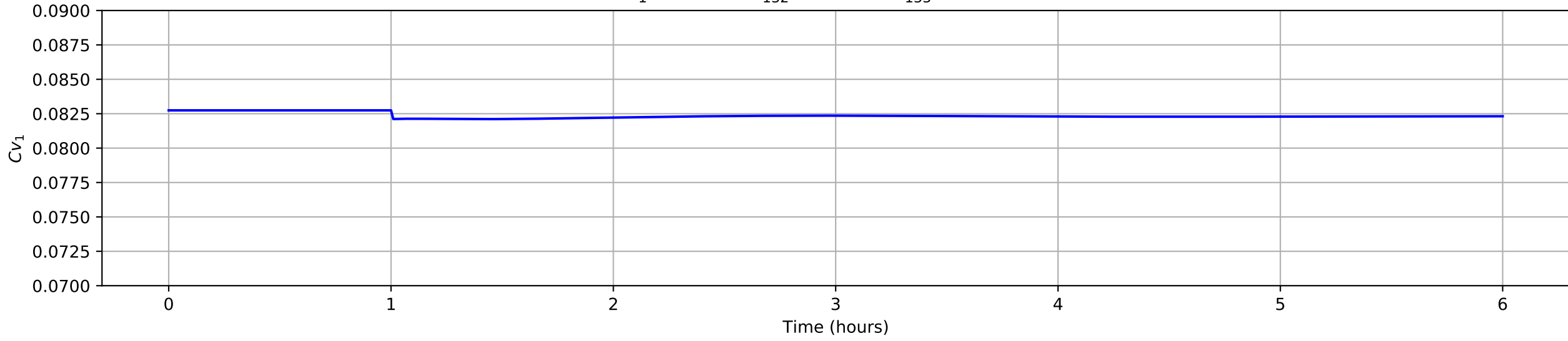
Disturbance: Increase of 5% in the feed flowrate. Cv_2 = 0.69671t_{132} + 0.69489t_{133} + 0.17807vf
