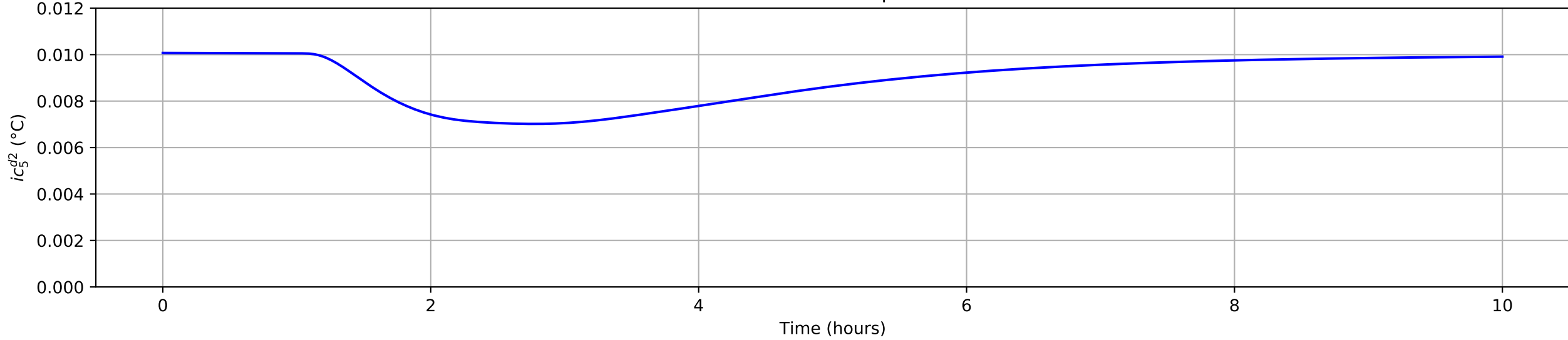
Disturbance: Decrease of 10% in the feed flowrate. IC5 Distillate composition
