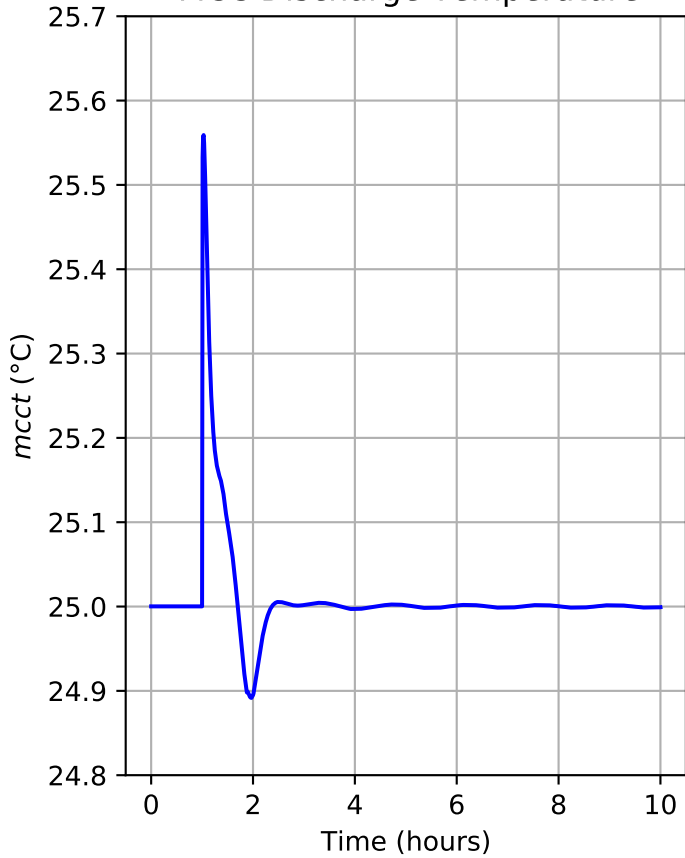
Disturbance: Increase of 5% in the feed flowrate. S8 Temperature
